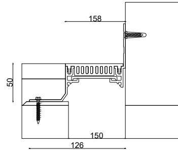
ZK-1175-75W79 H50
