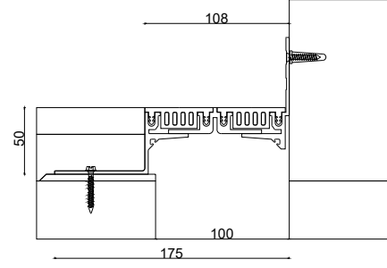
ZK-1175-100W108 H50
