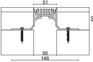
Z-1175-50W51 H50
