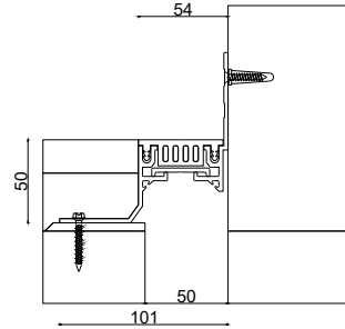
ZK-1175-50W54 H50
