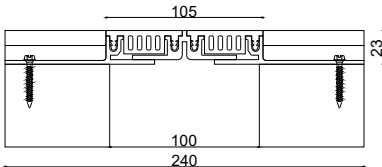
Z-1175-100W105 H23
