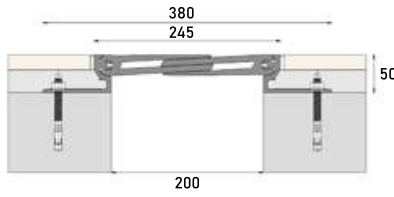
■ Z-1670A 200W245 JW :200 H:50 S:245 BW:380 M:100
