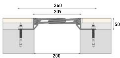
■ Z-1670A 200W209 JW :200 H:50 S:209 BW:340 M:100
