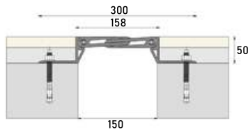
■ Z-1670A 150W158 JW :150 H:50 S:158 BW:300 M:60
