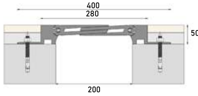
■ Z-1670A 200W280 JW :200 H:50 S:280 BW:400 M:80
