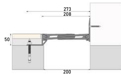
■ ZK-1670A 200W208 JW :200 H:50 S:208 BW:273 M:100
