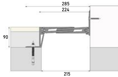
■ ZK-1670A 215W224 JW :215 H:90 S:224 BW:285 M:80
