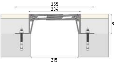
■ Z-1670A 215W234 JW :215 H:90 S:234 BW:355 M:80
