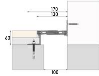
■ ZK-1670A 100W127 JW :100 H:60 S:127 BW:167 M:32
