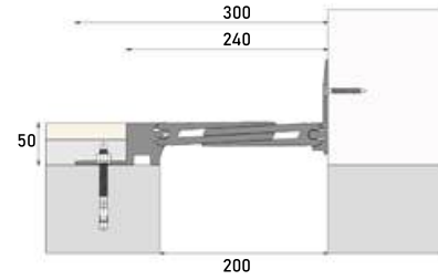
■ ZK-1670A 200W240 JW :200 H:50 S:240 BW:300 M:80
