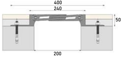
■ Z-1670A 200W240 JW :200 H:50 S:240 BW:400 M:80
