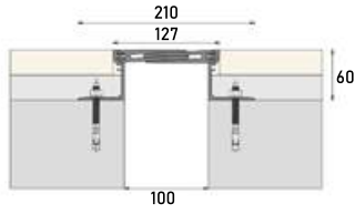
■ Z-1670A 100W127 JW :100 H:60 S:127 BW:210 M:32
