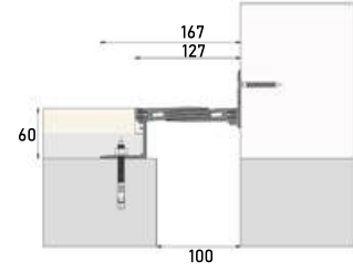
■ ZK-1670A 100W127 JW :100 H:60 S:127 BW:167 M:32
