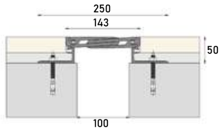
■ Z-1670A 100W143 JW :100 H:50 S:143 BW:250 M:32
